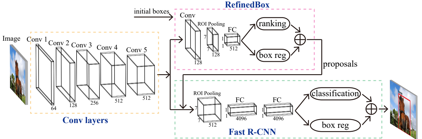
Figure 2: Overview of our network architecture. We display object detection as an example of joint training. The proposed network takes a nature image and corresponding initial boxes produced by other object proposal generation methods such as Edge Boxes as input. The branch of RefinedBox is designed to refine the initial boxes, then the refined boxes are inputted into the branch of Fast R-CNN for classification. Note that the refinement of boxes and consequent object detection can share the convolutional features.
