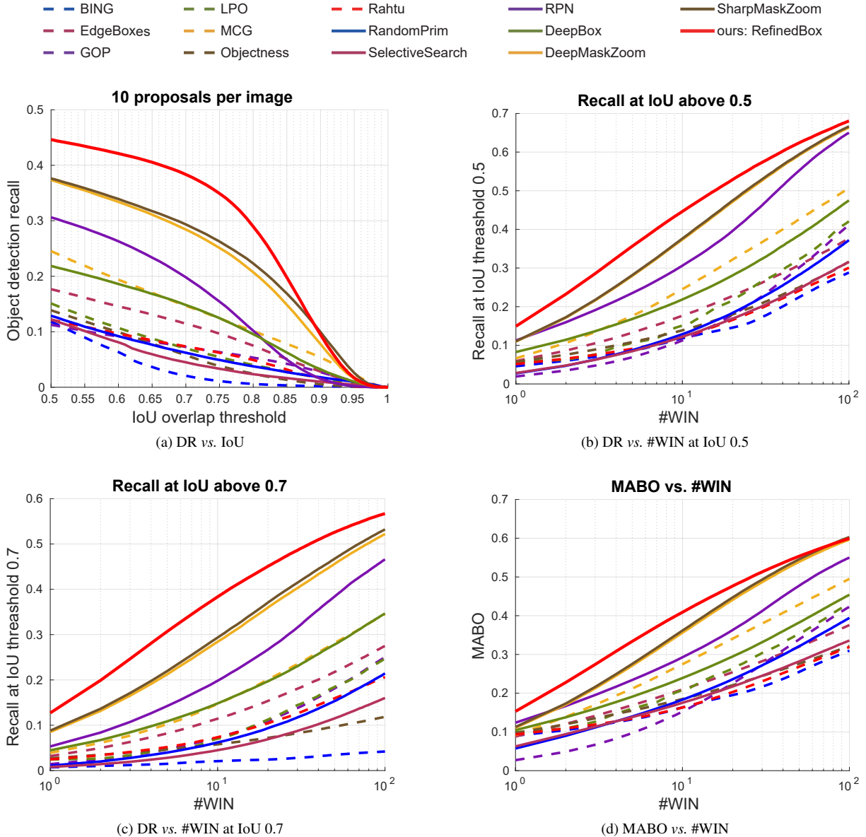
Figure 6: Evaluation results on the MS COCO validation set. RefinedBox uses RPN [13] as inputs. (a) shows object detection recall vs. IoU overlap threshold using 10 proposals per image. (b) and (c) display object detection recall vs. the number of proposals (#WIN) at IoU threshold 0.5 and 0.7, respectively. (d) shows MABO vs. the number of candidates using at most 100 proposals per image.
