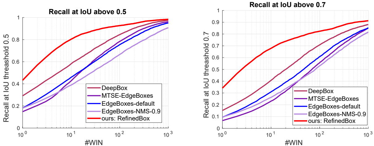
Figure 3: Evaluation of different refinement algorithms. These two subfigures show object detection recall vs. the number of proposals (#WIN) at IoU threshold 0.5 (left) and 0.7 (right), respectively. The method of EdgeBoxes-default is Edge Boxes [9] with default parameters, and EdgeBoxes-NMS-0.9 changes the parameter of non-maximum suppression (NMS) to 0.9.
