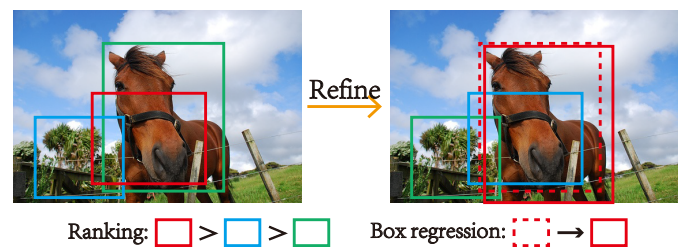
Figure 1: Overview of object proposal refinement. The left image shows the original proposals, and the right image shows the results after refinement. We first re-rank the proposals by computing new objectness scores, after which a box regression procedure is applied to each proposal box for accurate location.
