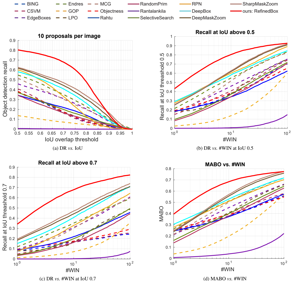
Figure 4: Evaluation results on the PASCAL VOC2007 test set. (a) shows object detection recall vs. IoU overlap threshold using 10 proposals per image. (b) and (c) display object detection recall vs. the number of proposals (#WIN) at IoU threshold 0.5 and 0.7, respectively. (d) shows MABO vs. the number of candidates using at most 100 proposals per image.
