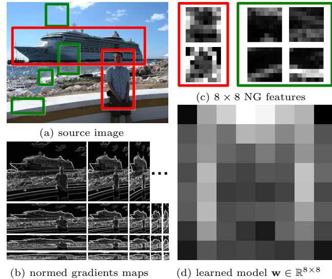
Fig. 1 Although object (red) and non-object (green) windows present huge variation in image space (a), at proper scales and aspect ratios which correspond to a small fixed size (b), their corresponding normed gradients, i.e. a NG feature (c), share strong correlation. We learn a single 64D linear model (d) for selecting object proposals based on their NG features.
